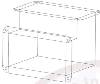
#14 Vertical 90-degree Ell
